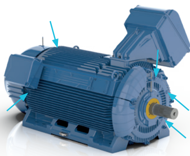
Figure 39 - Location of vibration measuring points.
