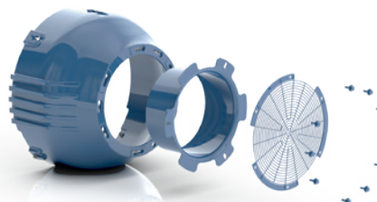
Figure 24 - Mounting system that ensures low noise levels.
