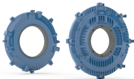
Figure 20 - DE endshield (left) and NDE endshield (right).
