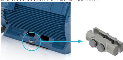
Figure 11 - Detail of the standard grounding terminal for the main terminal box and frame.
