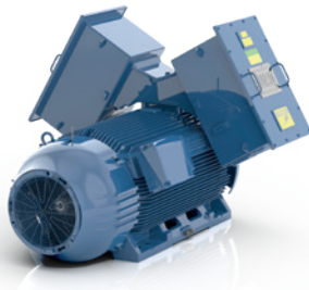
Figure 17 - Motor with access to neutral connection in separated terminal box.
