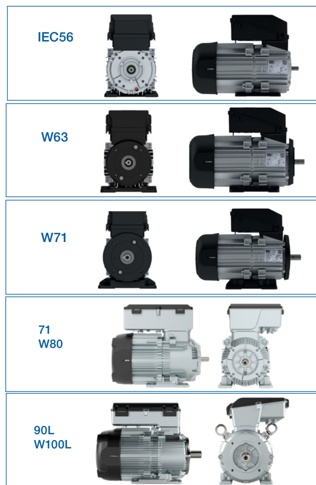
Figure 3 - W12 frame sizes.
