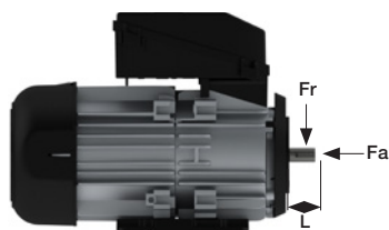
Figure 24 - Radial and axial force on the motor shaft
