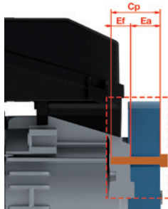
Figure 19 - Maximum threaded hole length
